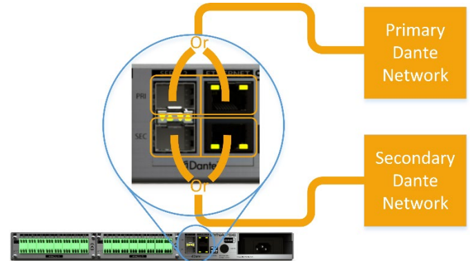
Figure 3 –“Redundant” mode, no daisy chain
